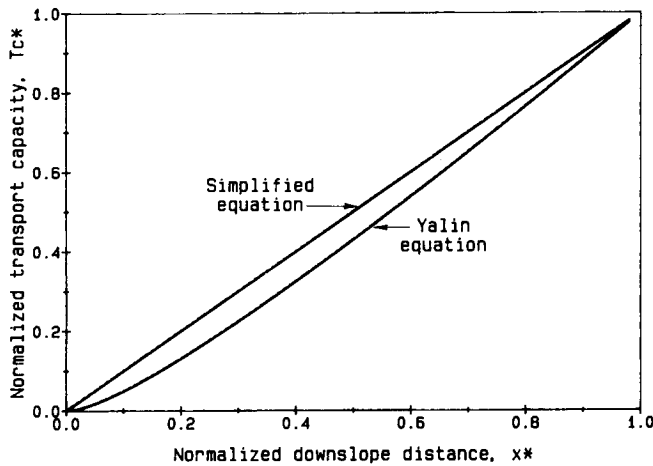
Fig. 4—A comparison of the simplified and Yalin transport capacity functions for profiles of various maximum transport capacities.
