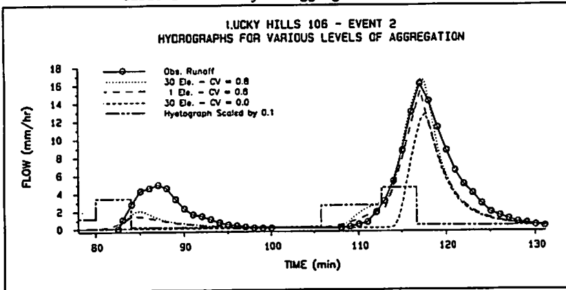
Figure 3 - Event 2 Hydrographs
