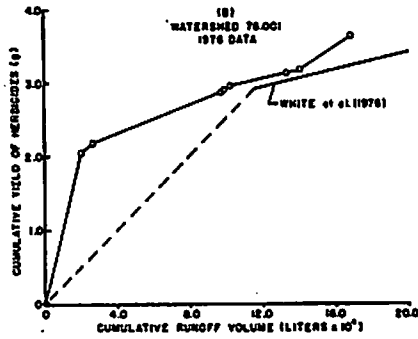
Figure - 4. Relation between runoff volume and herbicide yields.
