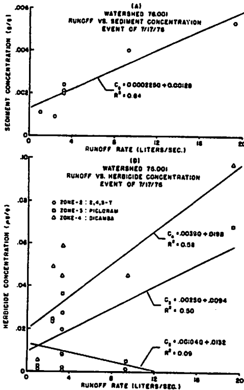
Figure - 6. Relations between runoff rate and concentration.
