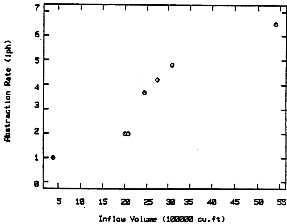
Figure 3. Abstraction versus inflow volume.
