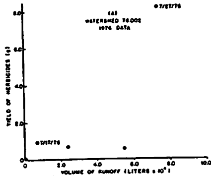
Figure - 4. Relation between runoff volume and herbicide yields.
