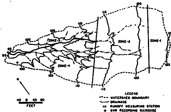
Figure - 2. Map of Watershed 76.002 showing drainage pattern and the division of the watershed into geomorphic zones.
