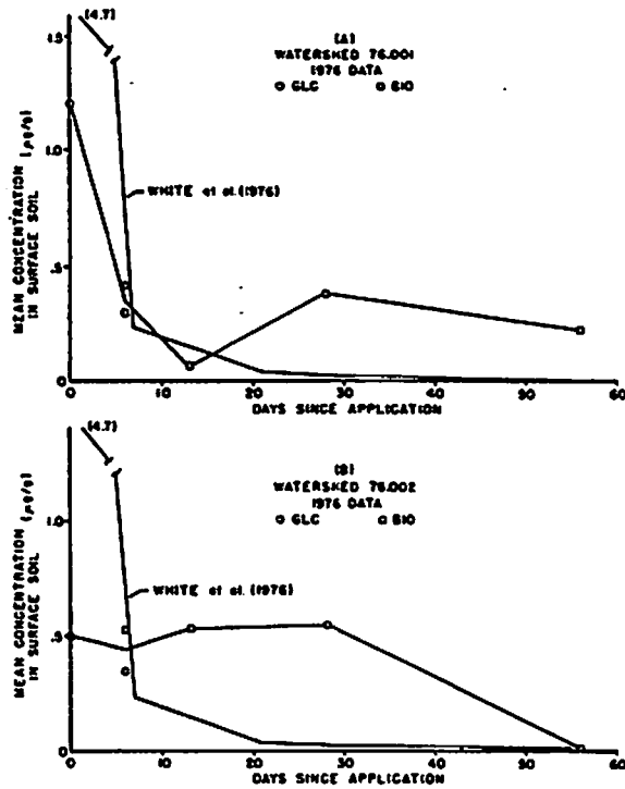
Figure - 3. Herbicide concentrations in surface soil. Initial application rate of 1.0 kg/ha. GLC represents concentrations by gas chromatography and BIO is the bio-assay method.
