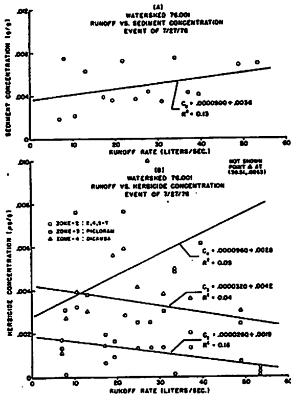
Figure - 7. Relations between runoff rate and concentration.
