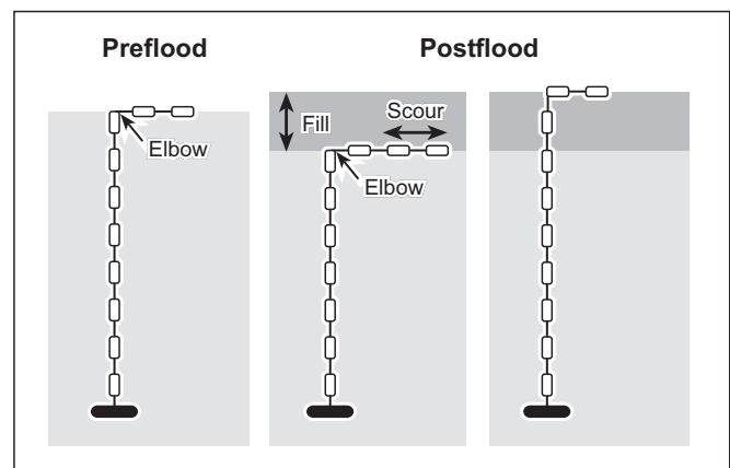
Figure 2. Schematic illustration of scour chain defining a net fill event.
