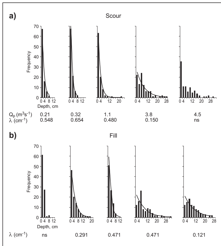
Figure 4. Frequency distributions of scour (a) and fill (b) for five runoff events in the main channel ( n = 96 ). Statistically significant exponential distributions are shown by the fitted lines (ns = not significant).
