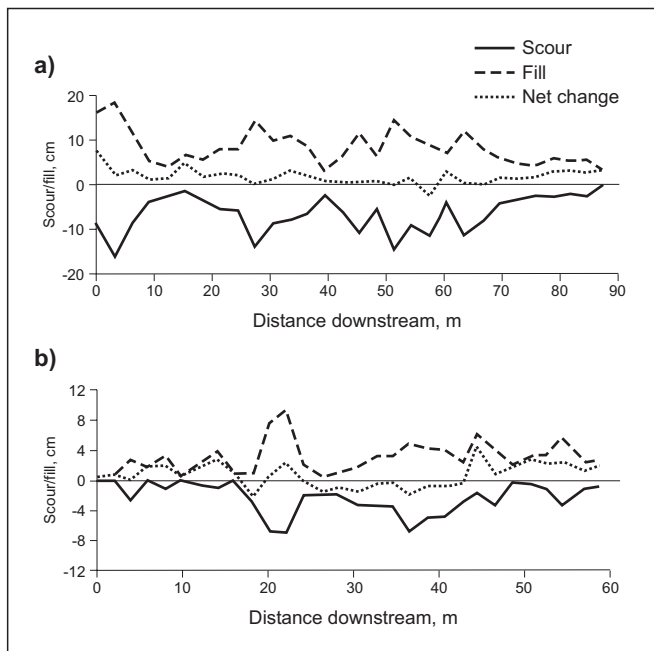
Figure 3. Spatial patterns of cross-sectional average scour, fill and net change in (a) the main channel ( Q_p = 4.5 \text{ m}^3 \text{ s}^{-1} ) and (b) the lower tributary reach ( Q_p = 0.2 \text{ m}^3 \text{ s}^{-1} ).
