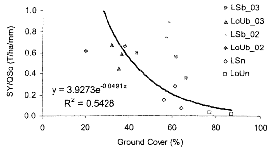
Fig. 2. Relationship between sediment yield ratio and percent ground cover.
