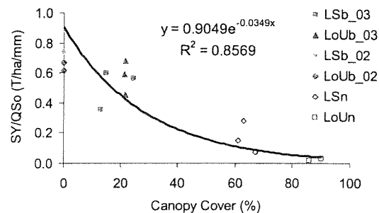
Fig. 3. Relationship between percent canopy cover and the sediment yield ratios.
