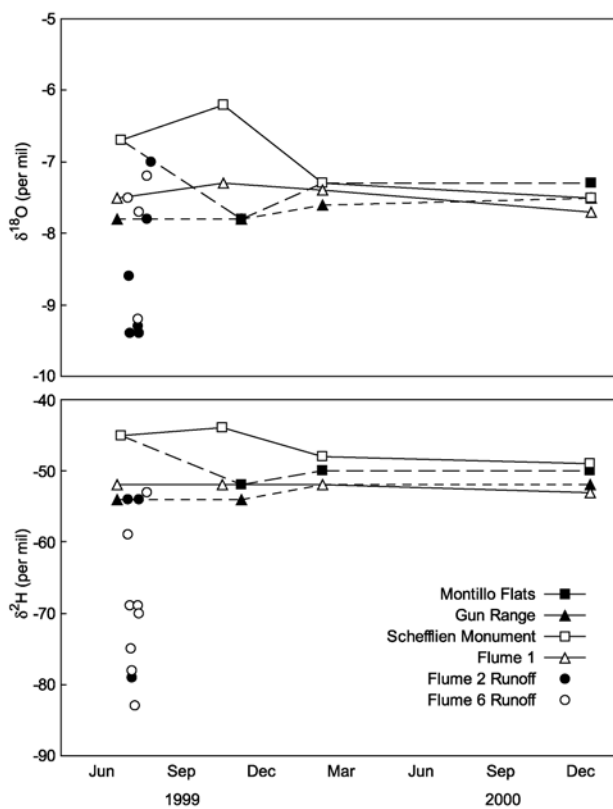
Figure 5. Oxygen and hydrogen composition of deep wells and runoff.
