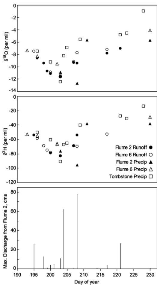
Figure 4. Oxygen and hydrogen isotope composition of rainfall and runoff during 1999, and maximum discharge rates at flume 2.
