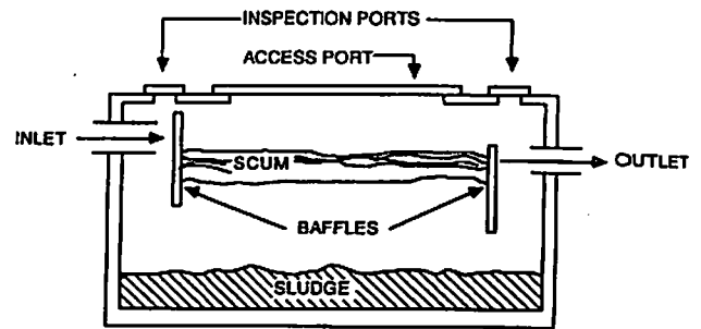
Figure S11 Components of a septic tank.
