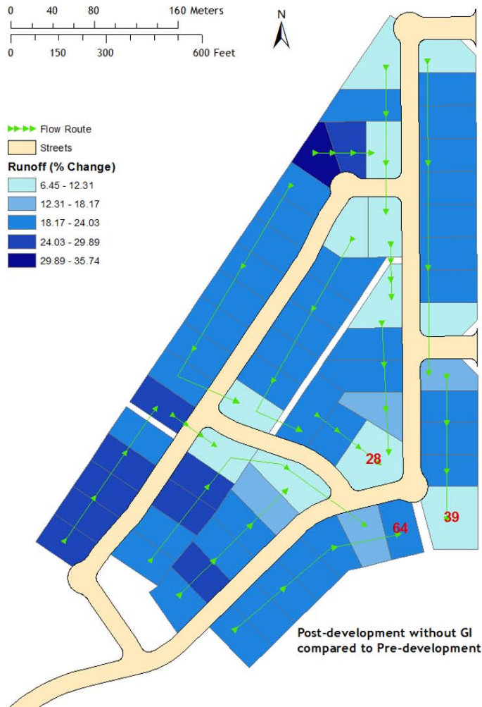
Figure 14: Percent Change in Runoff for Post-Development with and without GI Practices as Compared to Pre-Development.
