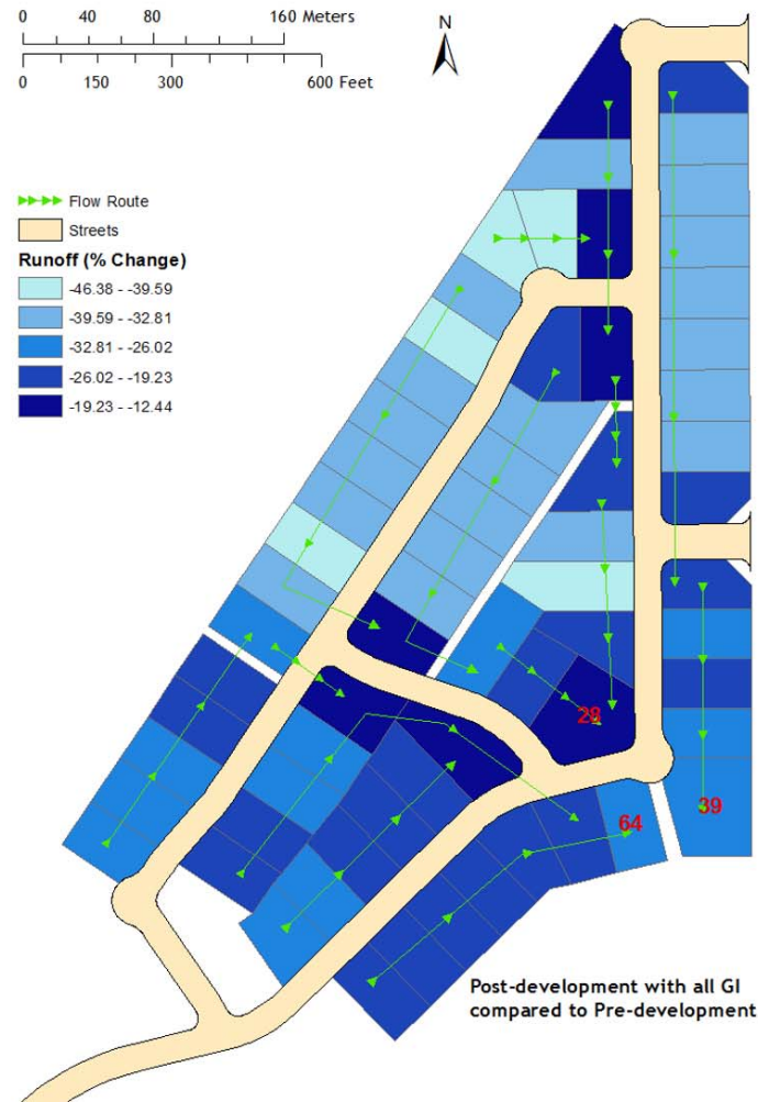
Figure 14: Percent Change in Runoff for Post-Development with and without GI Practices as Compared to Pre-Development.
