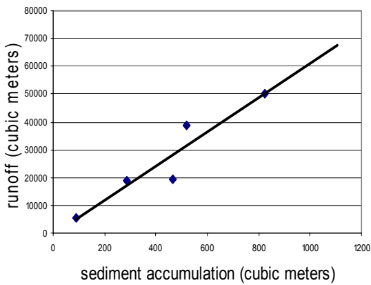
Figure 4. Relationship between runoff and sediment accumulation in Tank 63.223. R^2 = 0.90 .
